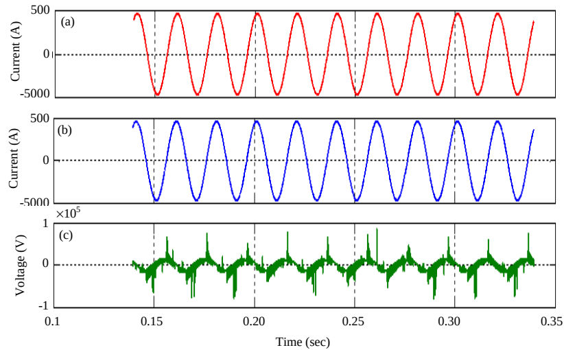
Fig. 5: Simulation results for VL1: a) Series measurement; b) Proposed technique and c) Inductor voltage
