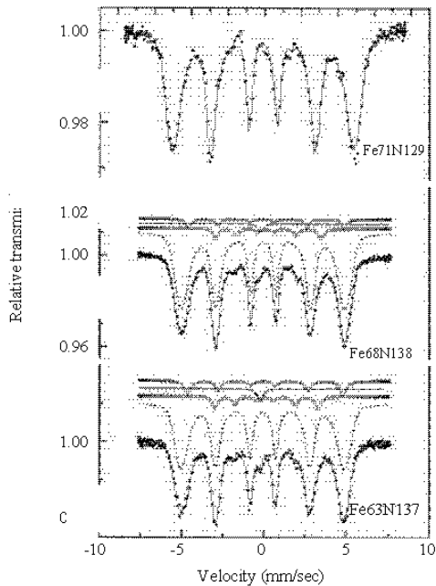
Fig. 3: Mossbauer spectra for the \text{Fe}_{100-x}\text{Ni}_x system (x = 29, x = 32 and x = 37)
