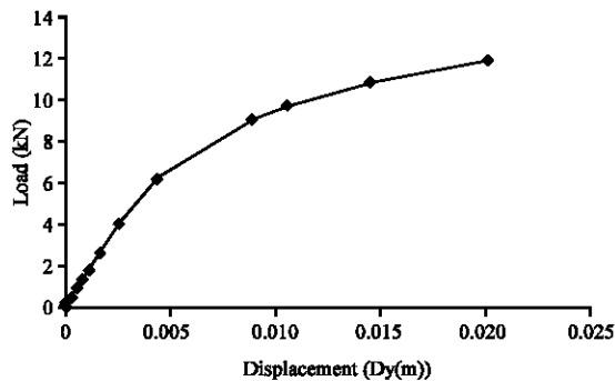
Fig. 13: Load-versus vertical displacement ( D_v ) at node 626 of specimen D.1/2-1
