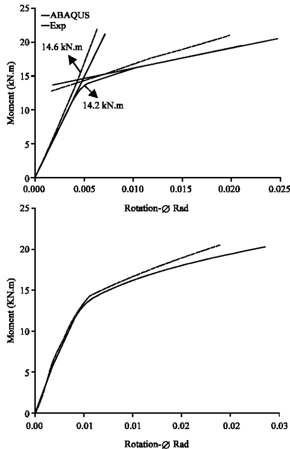
Fig. 18: Moment-rotation (M- \theta ) curve for specimen B.1/2-1
