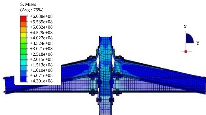
Fig. 10: Deformation of connection plot of spacieman D.1/2-1
