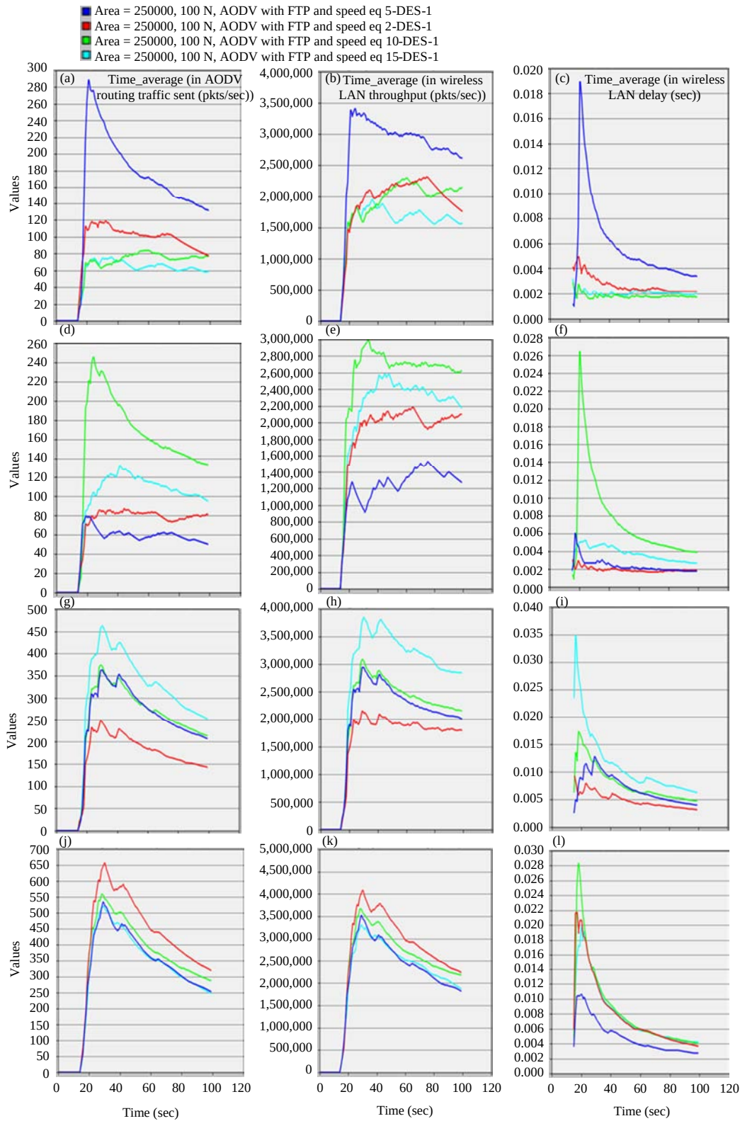
Fig. 4: Results of simulation using OPNET editor: a-c) Area is 500 \times 500 \text{ m}^2 , d-f) Area is 1000 \times 1000 \text{ m}^2 , g-i) Area is 1500 \times 1500 \text{ m}^2 and j-l) Area is 2000 \times 2000 \text{ m}^2
