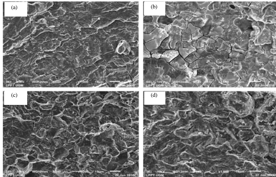
Fig. 12: SEM photographs of fractured surfaces of welded specimen tested in: a) Air; b) 3.5% NaCl; c) 3.5% NaCl+0.5% \text{Na}_2\text{Cr}_2\text{O}_4 and d) 3.5% NaCl+0.5% \text{Na}_2\text{MoO}_4
