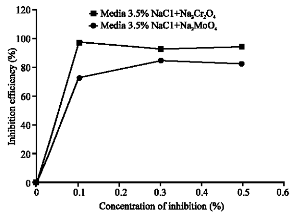
Fig. 5: Inhibitor efficiency
