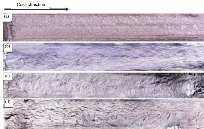
Fig. 11: Macro photographs of fractured surfaces of welded specimen tested in: a) Air ; b) 3.5% NaCl; c) 3.5% NaCl+ 0.5% \text{Na}_2\text{Cr}_2\text{O}_4 and d) 3. 3.5% NaCl+0.5% \text{Na}_2\text{MoO}_4
