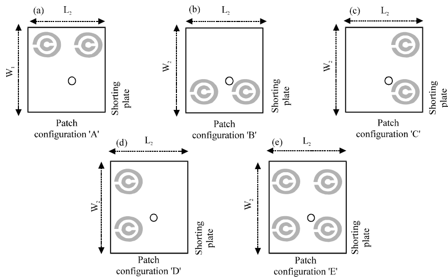
Fig. 3: Geometrical structure of SRR configurations 'A-E': a and b) 2 \times 1 SRR array; c and d) 1 \times 2 SRR array; e) 2 \times 2 SRR array
