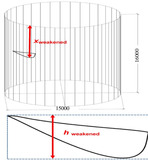
Fig. 3: Approximation of the weakened area by corrosion, determining h_{\text{weakened}} , determining the elevation coordinate of the weakened area x_{\text{weakened}}
