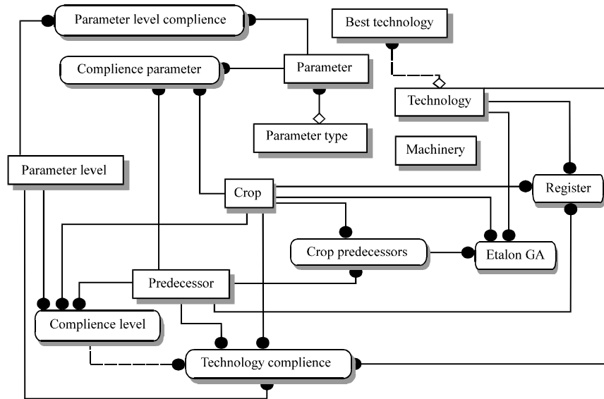
Fig. 3: ER-Model of constructed database
