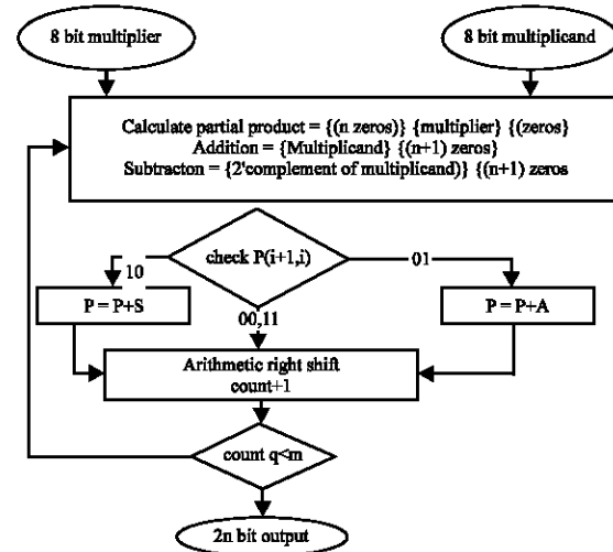
Fig. 1: Flow chart of Booth's multiplier
