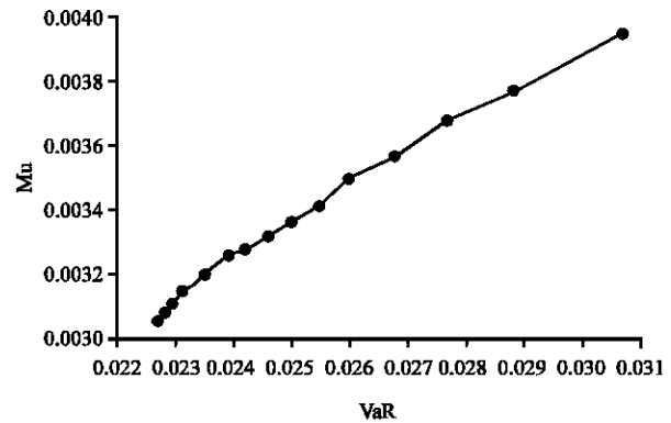
Fig. 1: Graphic of efficient portfolio Mean-VaR
