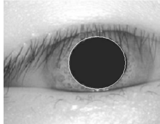
Fig. 7: Pupil detection
