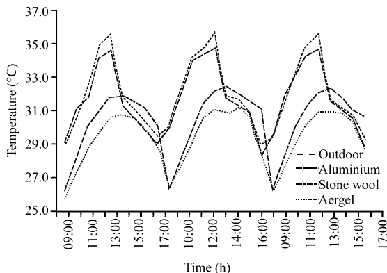
Fig. 11: Outdoor-indoor temperature profiles of the experimental houses
