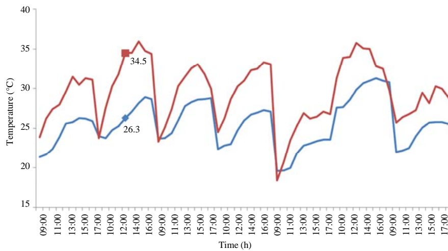
Fig. 9: Outdoor-indoor temperature profile for Aerogel-Insulated Model
