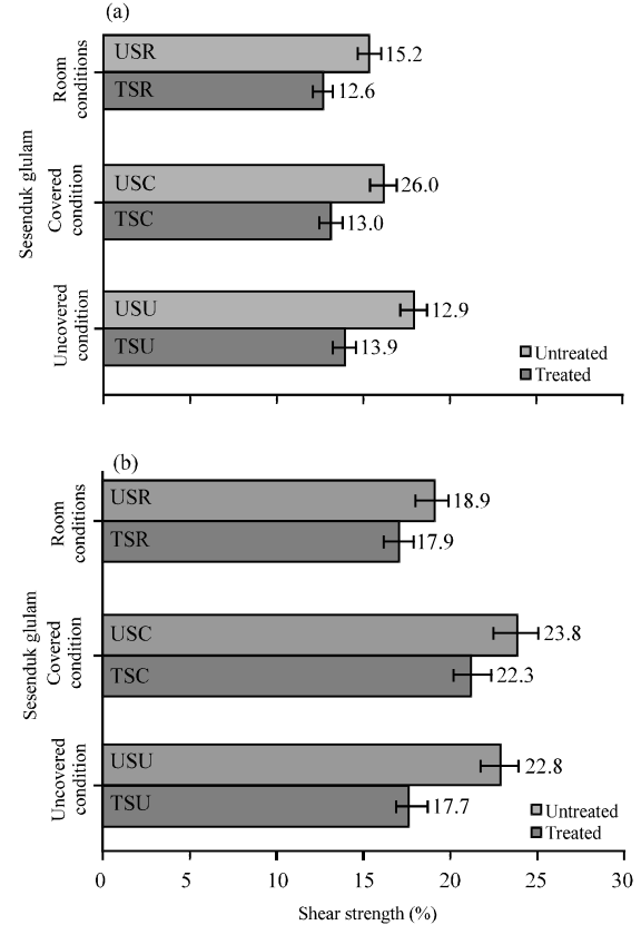
Fig. 3: Shear bond strength for: a) Sesenduk and b) Binatangor glulam under different exposures
