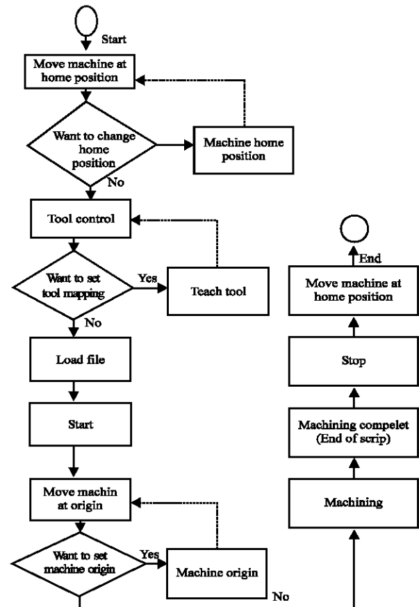
Fig. 3: Flow chart of developed system algorithm design
