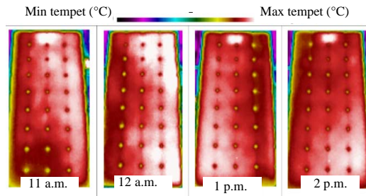
Fig. 4: Temperature distribution over the front surface of PV panel
