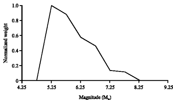
Fig. 2: Cumulative diagram for earthquake magnitude by Ambraseys et al. (2005)'s relation
