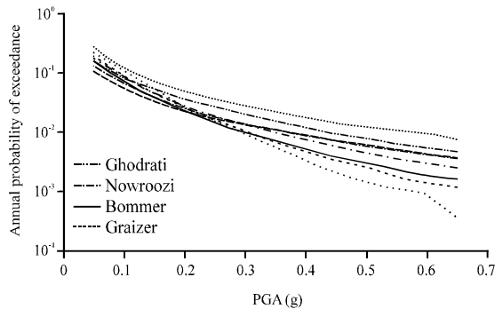
Fig. 11: Comparison of the new method's hazard curve with that of individual GMPE for Baghershahr region
