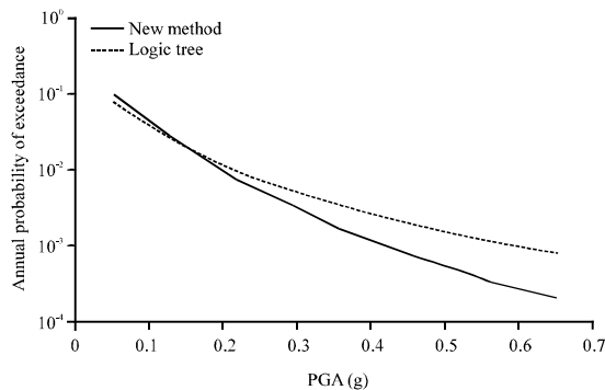
Fig. 12: Comparison of the new method's hazard curve with that of the proposed logic tree for Baghershahr region
