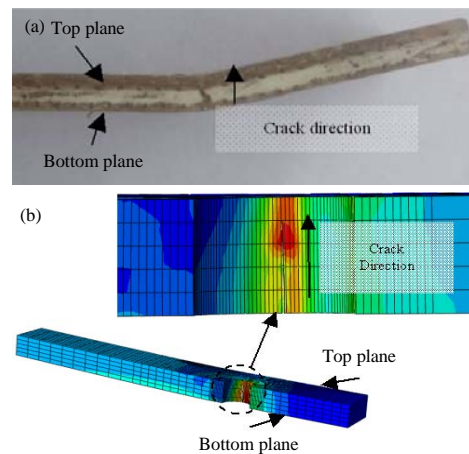
Fig. 4: Crack propagation through thickness from bottom plane to top plane in single lay-up: a) Experimentally and b) XFEM
