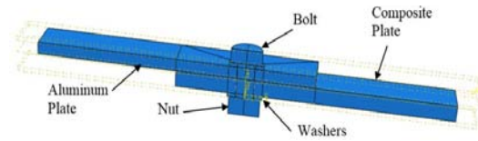
Fig. 2: Part components in single-lap joint implement in XFEM
