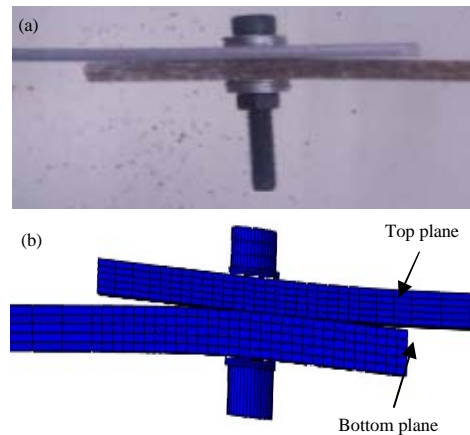
Fig. 3: Secondary bending in single-lap joint: a) Experimental observations and b) XFEM model
