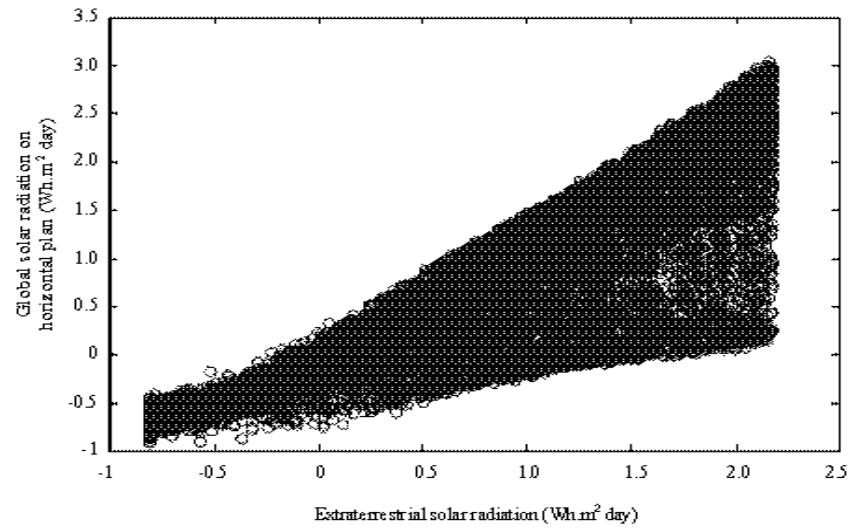
Fig. 12: Correlation between global solar radiation and extraterrestrial solar irradiation
