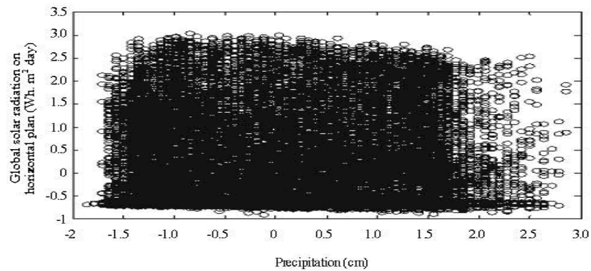
Fig. 14: Correlation between global solar radiation and precipitation
