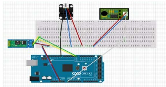
Fig. 2: Arduino architecture
