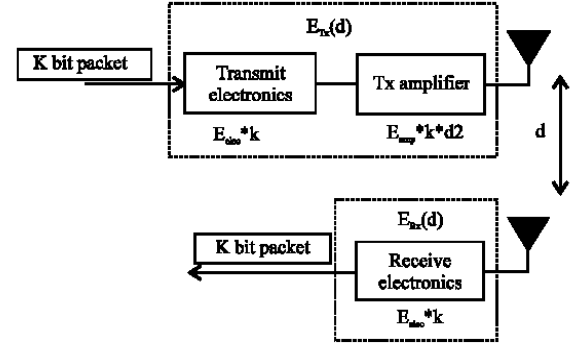
Fig. 2: Radio model
