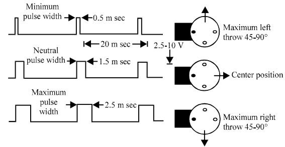
Fig. 6: Servo motor pulse width (Richling, 2012) www.mitchr.me
