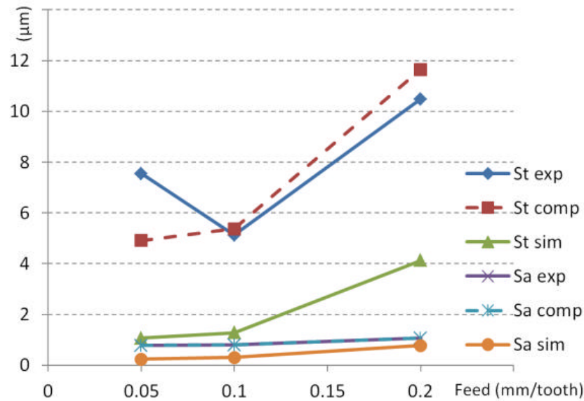
Fig. 8: Comparison of the experimental, simulated and compensated areal roughness of the ball end mill
