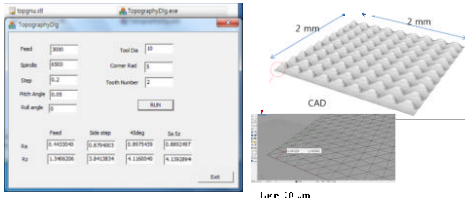
Fig. 2: Micro surface topography prediction software
