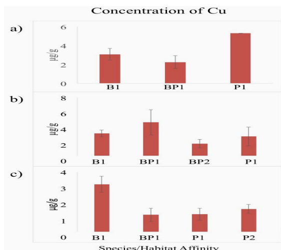
Fig. 2: Concentration of copper, Cu in benthic (B), Benthopelagic (BP) and pelagic fishes based on different organs: a) gills, b) liver, c) muscles. B1 = C. macrolepidotus , BP1 = E. tauvina , BP2 = A. thalassinus , P1 = P. erumei , P2 = C. macrolepidotus
