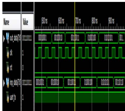
Fig. 6: Receiver results of UART
