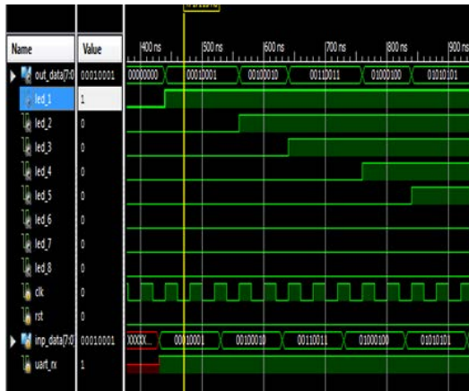
Fig. 6: Receiver results of UART
