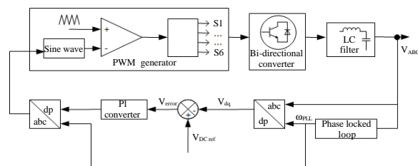
Fig. 5: Basic block diagram of the voltage control method
