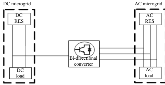
Fig. 1: Schematic diagram of the AC-DC microgrid
