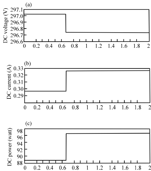
Fig. 6: DC system isolated mode; a) DC voltage; b) DC current and c) DC power
