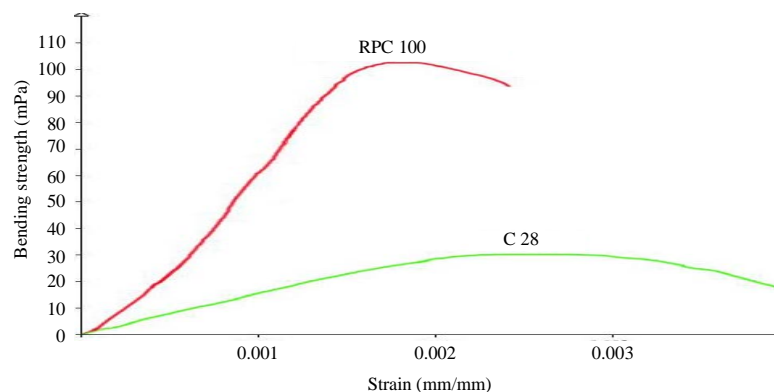
Fig. 5: A diagram of mechanical behavior in powder concrete sample of optimal plan (plan 3) compared with usual concrete sample (28 mPa)
