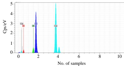
Fig. 8: C.S ratio in the paste available in plan 1 is equal to 1.9 which shows presence of higher amounts of type III gel C-S-H in powder concrete matrix
