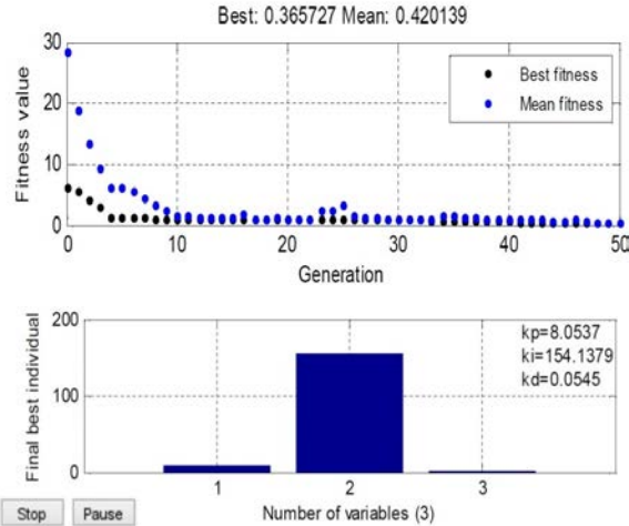
Fig. 6: GA optimization progression based objective function (MSE) performance index
