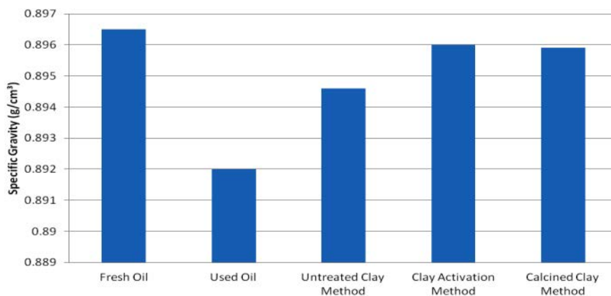
Fig. 6: Effect of recycling of waste used lube oil on its specific gravity
