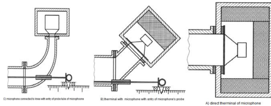
Fig. 4: different types of microphone base
