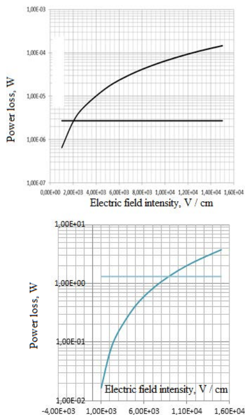
Fig. 2: Analysis of power losses for the dielectric heating of micro-organisms: a) water; b) fat) at different electric field intensities and heat losses power at cyclical fat temperature excess to 70°C
