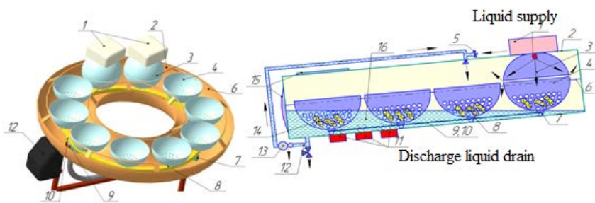
Fig. 4: Installation with ultrasonic and microwave generators for treatment of fat-containing raw materials (spatial and schematic picture); 1: microwave generator with magnetron; 2: circular waveguide; 3: stationary hemisphere of the cavity resonator; 4: movable perforated hemisphere cavity; 5: liquid supply pipe; 6: directing bezel; 7: rollers; 8: articulation; 9, 10: driving sprocket with gear ring; 11: piezoelectric elements of the ultrasonic generator; 12: branch pipe to drain the waste liquid; 13: circulation pump with filter; 14: fat-containing raw material; 15: door for unloading and loading a raw material; 16: washing fluid
