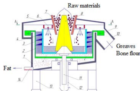
Fig. 7: Design of the microwave installation for separation of molten fat from fat containing raw materials; 1: cylinder-shaped shielding enclosure; 2: perforated cylindrical rotor; 3: cylindrical drum; 4: auger; 5: shielding enclosure cover; 6: MW generator unit with the magnetron radiator; 7: charging capacity; 8: conical radiation limiter; 9: scrapers; 10: product discharge pipe; 11: rotor, drum and auger shaft; 12: hollow shaft of the rotor; 13 mounting rack
