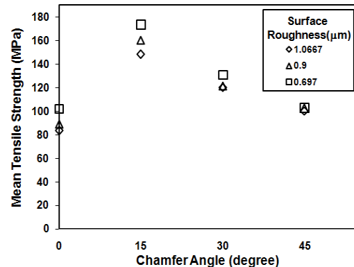
Fig. 12: Relationship of surface roughness, chamfer angle and tensile strength of A6061 CDFW joint
