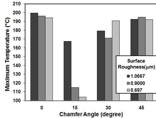
Fig. 11: Maximum temperature on the middle-outer flash of CDFW joints with various chamfer angle and surface roughness
