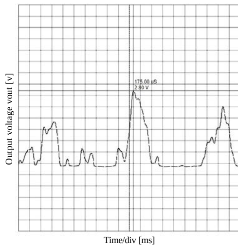
Fig. 4: The output signal of adder circuit for audio signal with 280 mV an amplitude
