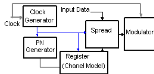
Fig. 1: Sender structure
