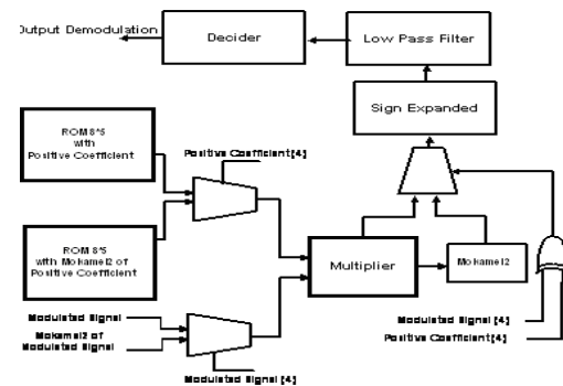
Figure 5: Modulator structure
