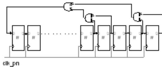
Fig. 1: Sender structure
