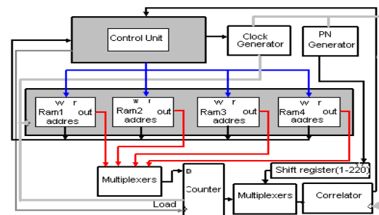
Fig. 8: Memory unit
