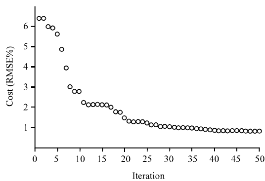
Fig. 22: Iterations
