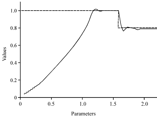
Fig. 12: Motor speed with fuzzy control type-1
