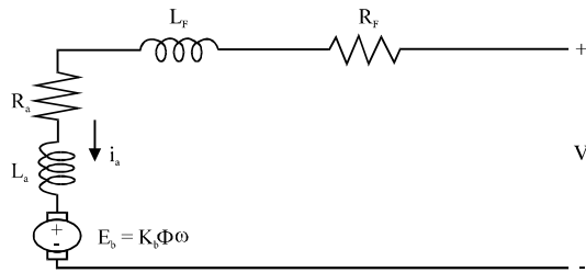
Fig. 7: DC motor shunt circuit
