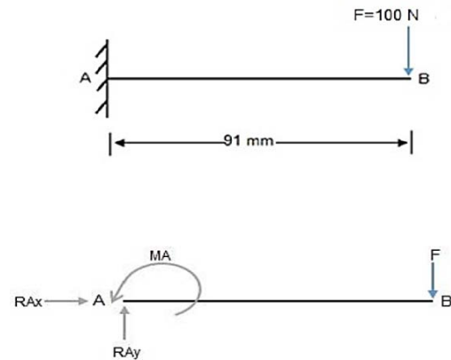
Fig. 8: The hand body is assumed as a cantilever beam
