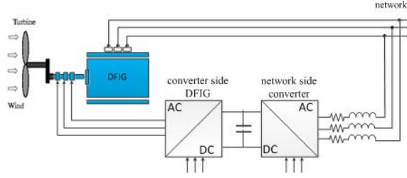
Fig. 1: Wind turbine system based on DFIG
