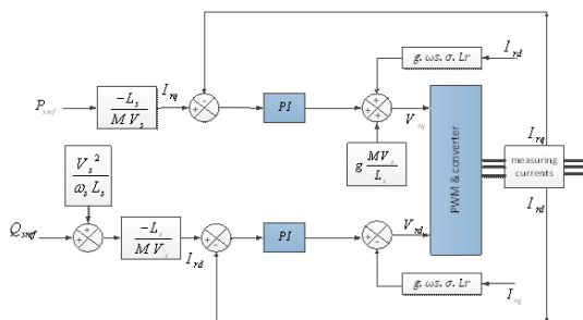
Fig. 2: Simplified DFIG model
