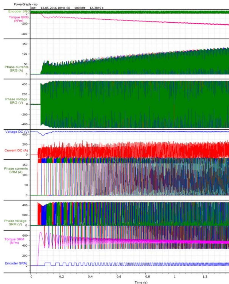
Fig. 5: Acceleration oscillogram
