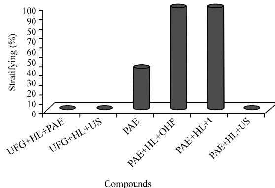
Fig. 2: The histogram of the dependence of glued solid timber slat separation after the cyclic tests (ret-drying)
