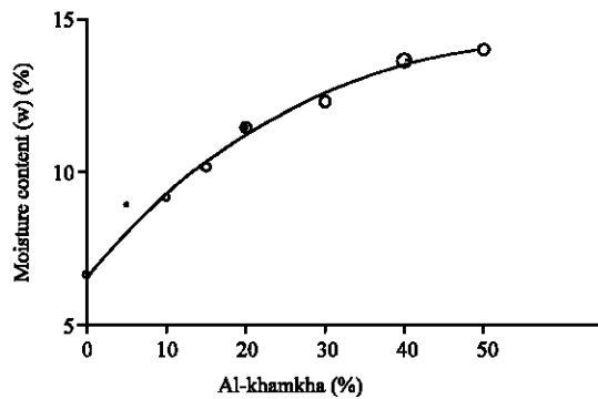
Fig. 3: Effect of Al-kamkha on the compaction characteristic of Jerash cohesive soil
