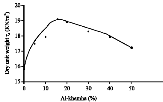
Fig. 2: Effect of al-kamakha on the compaction characteristic of Jerash cohesive soil
