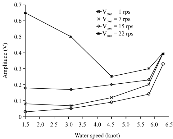
Fig. 9: Amplitude range of propeller noise for B-series 4-blade propeller at P = 1.4 bar for various propeller velocities
