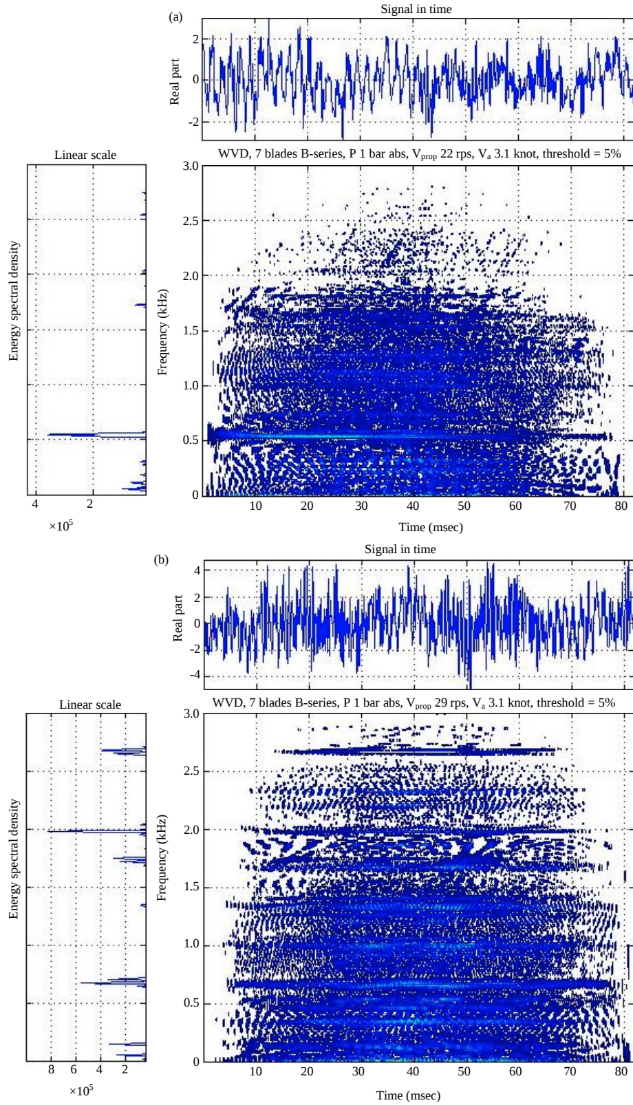
Fig. 16: The WVD representation of the acoustic noise in the tunnel when B-series 7-blade propeller, V_{water\ in\ the\ tunnel} = 3.1 knot and P_{in\ the\ tunnel} = 1.0 bar
