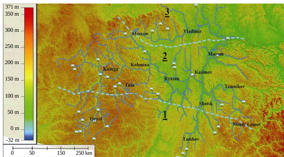
Fig. 2: Hydrological regions
