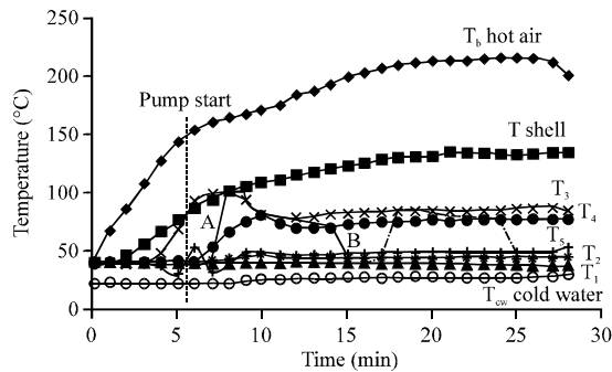
Fig. 7: Relationship between temperature and time of pasteurization ( T_1 = 33^\circ\text{C} , flow rate 806\text{ mL min}^{-1} ; T_b = 210^\circ\text{C} ): T_1 = Raw milk; T_2 = After preheating; T_3 = Pasteurization; T_4 = Before cooling; T_5 = Post colling
