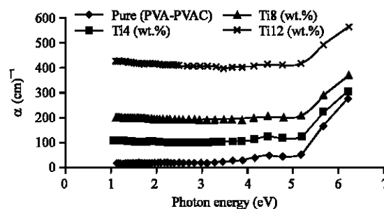
Fig. 2: The variation of absorption coefficient for (PVA-PVAC-Ti) nanocompsites with photon energy
