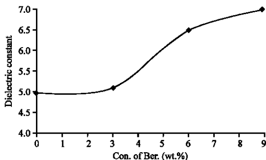
Fig. 14: The variation of the dielectric constant of biocomposites with the concentration of berry paper mulberry
