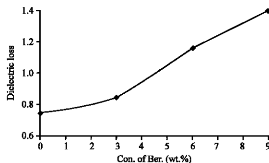
Fig. 16: The variation of the dielectric loss of biocomposites with the concentration of berry paper mulberry at 100 Hz
