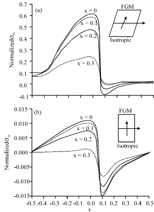
Fig. 11: Normalized stress distribution through different locations for FG; a) Simply supported; b) Clamped-clamped (\gamma = 10, h = 0.1)
