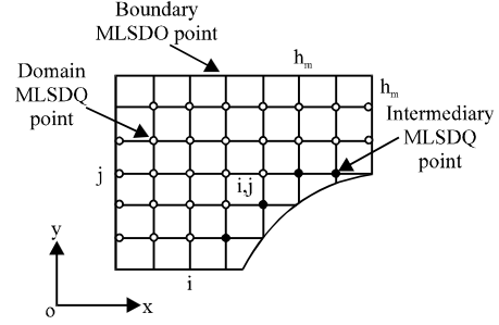
Fig. 2: Grid discretization for the hybrid technique consisting of FDM and MLSDQM
