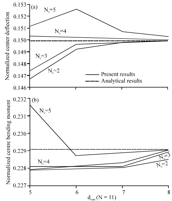
Fig. 4: Variation of the results with the radius of support domain and completeness order for a regular discretized clamped-clamped plate ( N_1 = 11 ); (Reddy, 1999, 2002; Timoshenko and Woinowsky-Krieger, 1959)
