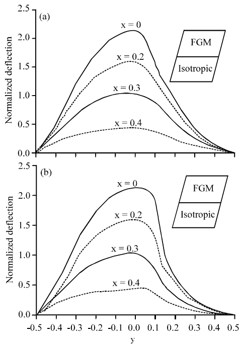
Fig. 9: Normalized deflection distribution through different locations for FG simply supported skew plate: a) (\gamma = 1) ; b) (\gamma = 10)
