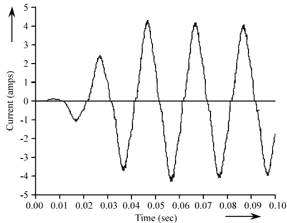
Fig. 10: Grid current
