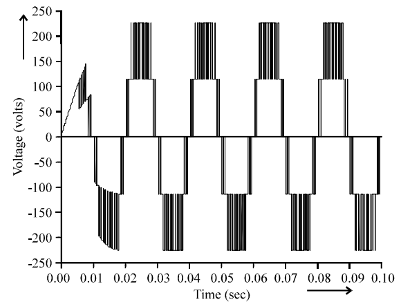
Fig. 9: Proposed inverter output voltage
