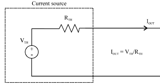
Fig. 1: Current source
