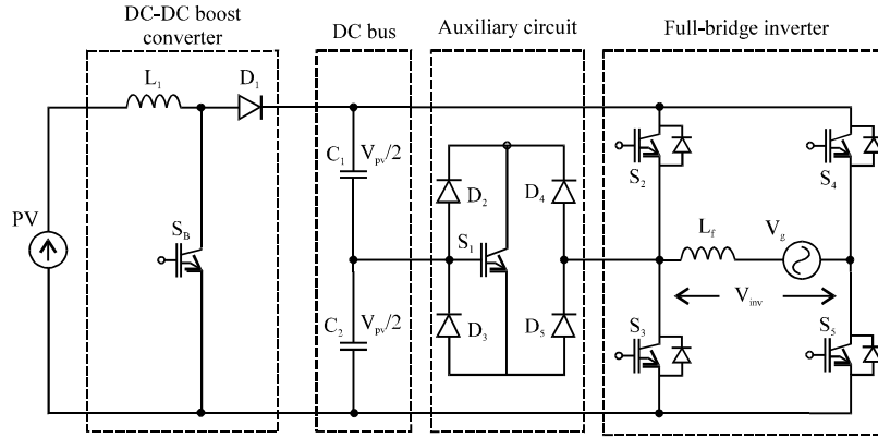
Fig. 5: Proposed inverter topology
