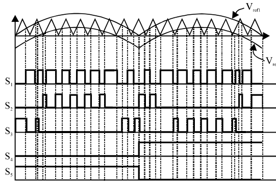
Fig. 6: Switching pattern for the single-phase five level inverter
