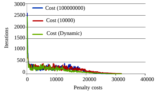
Fig. 2: Behavior of SA-D compared to SA that use a static initial temperature for Comp 1
