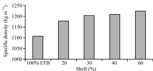
Fig. 4: Specific density ( \text{kg m}^{-3} ) of palm briquettes at different shell ratio (%)
