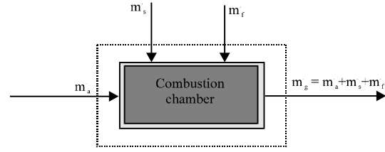
Fig. 2: Control volume of combustion chamber (Application of mass balance)
