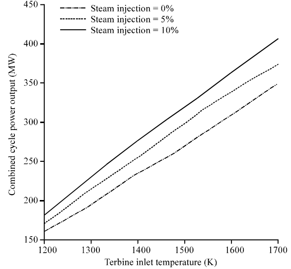
Fig. 9: Effect of turbine inlet temperature on the combined cycle power output with various amount of steam injection
