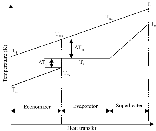
Fig. 3: Schematic of heat recovery zones
