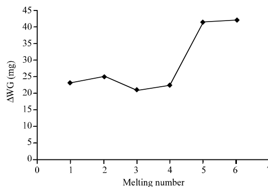
Fig. 3: Effect of different terms of making ferrite (melting number) on acid resistance of lead glass samples
