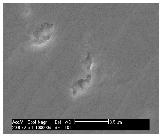
Fig. 6: Scanning electron microscopic images of glass sample (G4) after 2 h heat treatment (100000 X)
